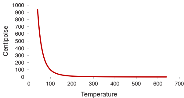
Dynamic Viscosity
