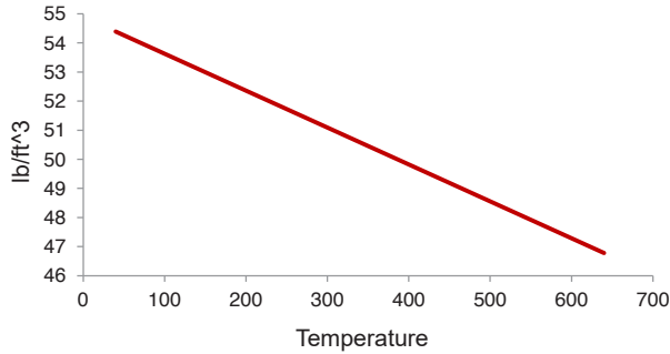
Density
